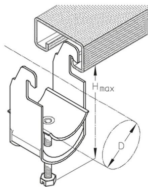
44AC-AL
