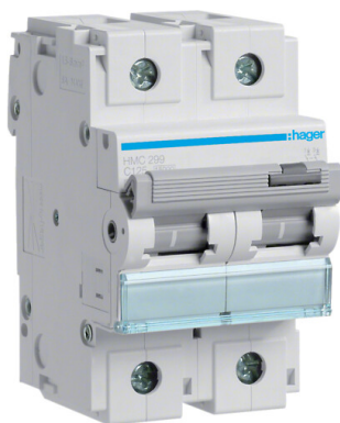
HMC299
