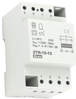
ZTR-15-12V
